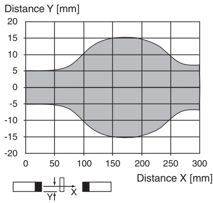
Obstacle: flat plate 100 mm x 100 mm
